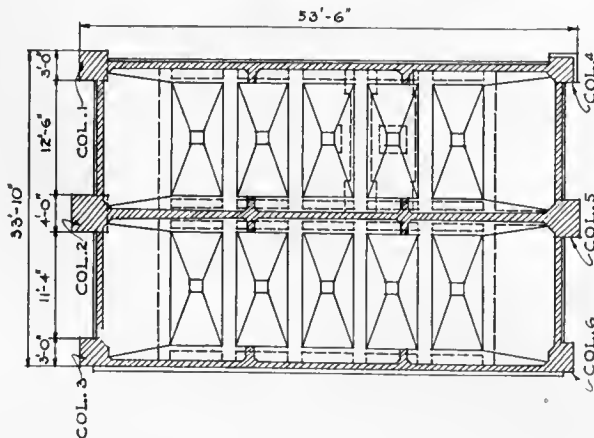
SECTION G-G. FLOOR OF BIN, SHOWING HOPPERS
